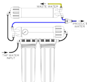
Figure 1: Installation of Piggyback Kit
