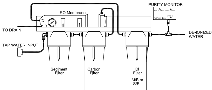
TYPICAL 4-STAGE RO/DI SYSTEM
